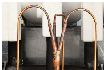
Expansion Device-Capillary
