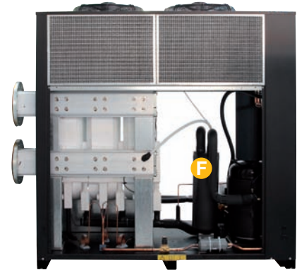
Large-volume liquid separator F
